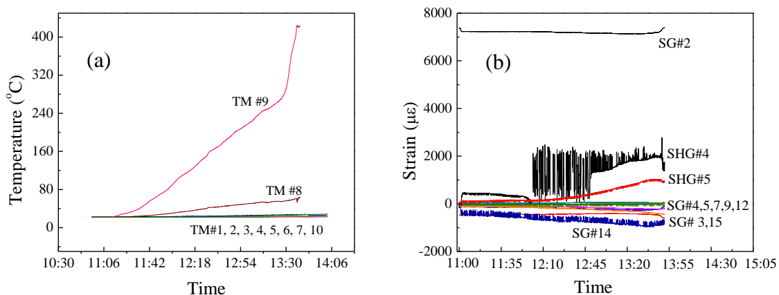
Figure 4.17 Changes monitored by commercial sensors: (a) temperature ( F = C \times 9/5 + 32 ) and (b) strain
