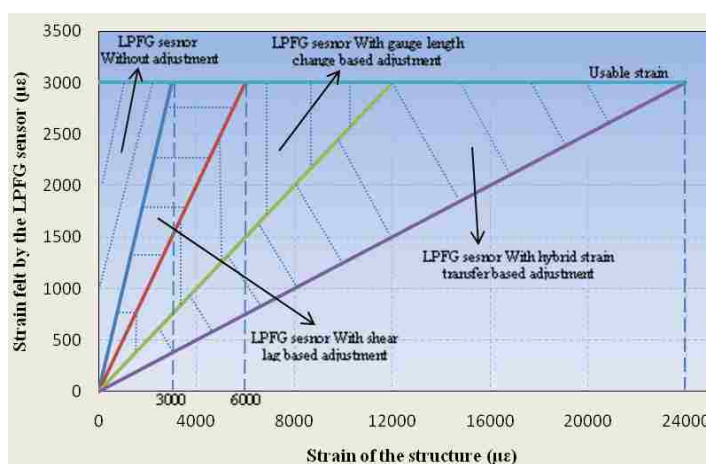
Figure 3.9 Effects of various strain transfer mechanism
