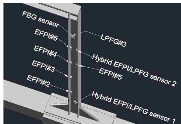
Figure 4.8 Specific locations of fiber optical sensors in three-dimensional view
