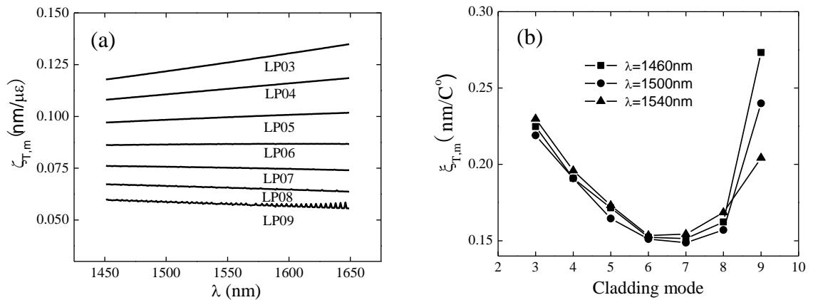
Figure 3.3 Temperature sensitivity \xi_{T,m} : (a) function of center wavelength and (b) relation with cladding mode
