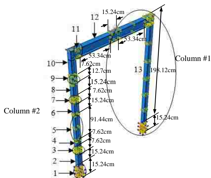
Figure 5.11 FEM of the steel frame and temperature zones
