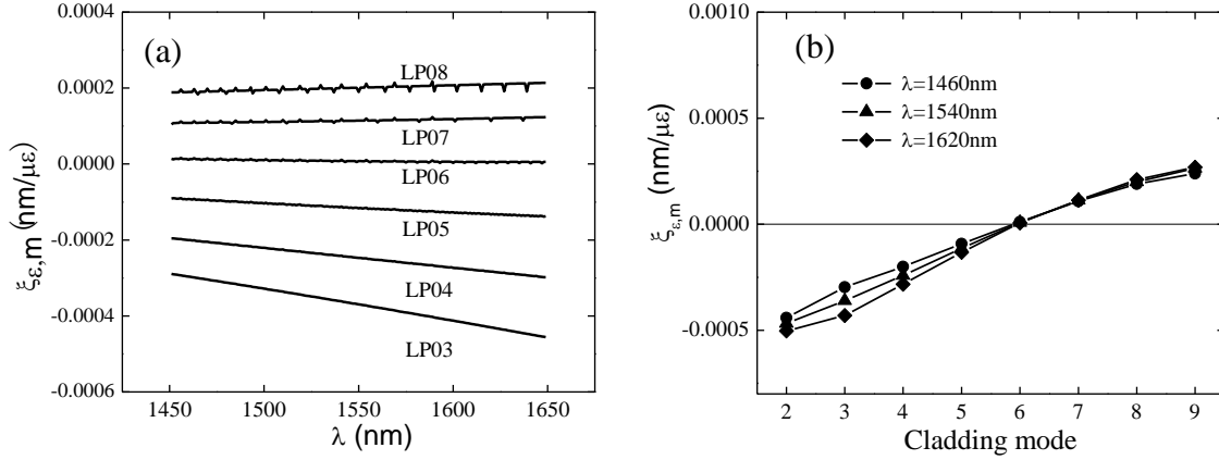
Figure 3.4 Strain sensitivity \xi_{\varepsilon,m} : (a) function of center wavelength and (b) relation with cladding mode
