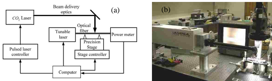
Figure 3.1 LPFG fabrication: (a) a CO 2 laser system and (b) processing units
